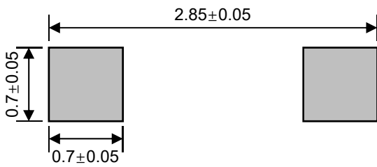
Suggested PCB Layout
