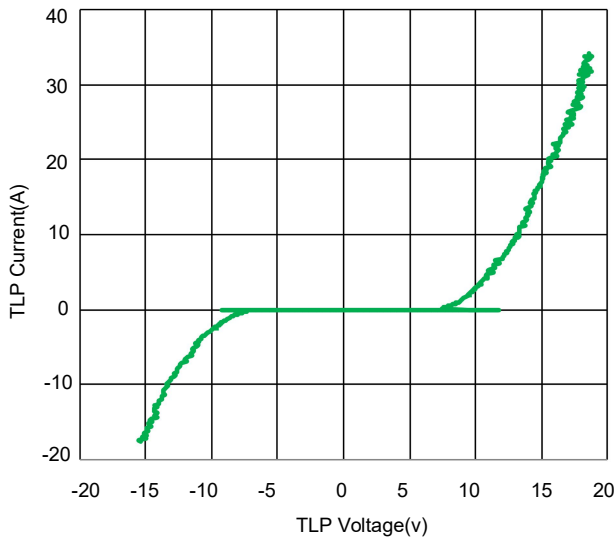
Fig 5. TLP Measurement
