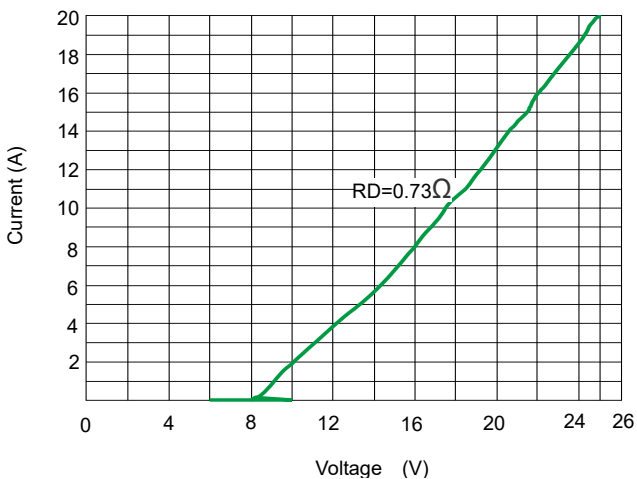
Fig 5. TLP Measurement
