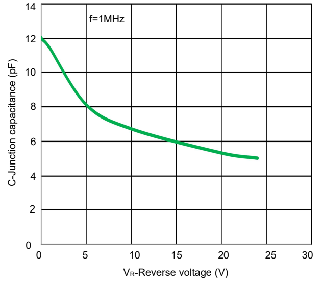
Fig 4. Capacitance vs. Reverses voltage
