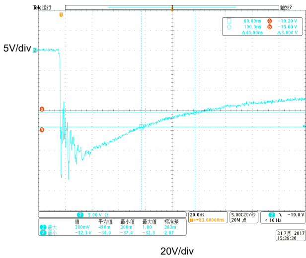
Fig 9. ESD clamping voltage (IEC61000-4-2-8KV contact)
