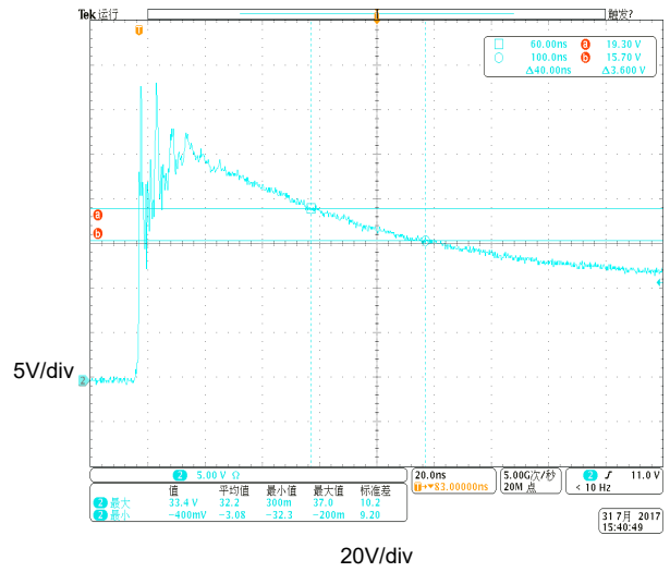
Fig 8. ESD clamping voltage (IEC61000-4-2 +8KV contact)
