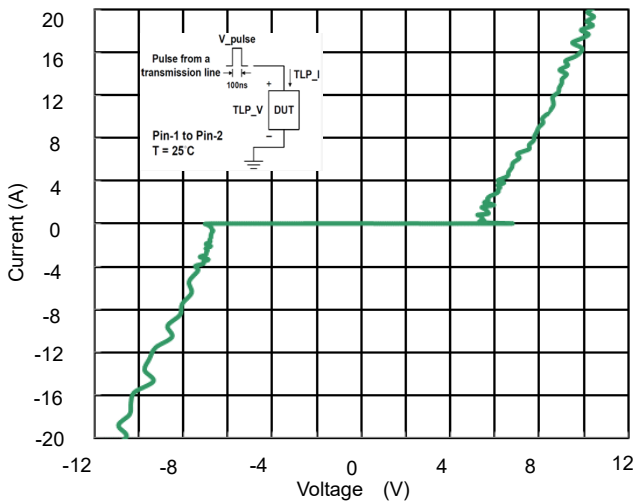
Fig 3. TLP Measurement
