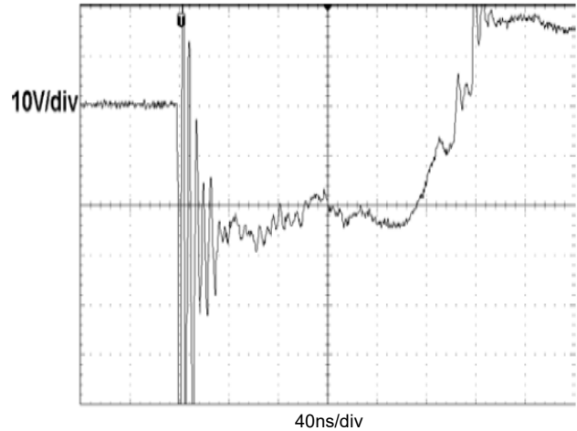
Fig 8. ESD clamping voltage (IEC61000-4-2-8KV contact)
