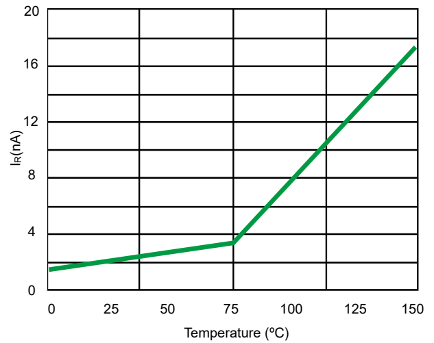
Fig 4. Typical Leakage Current vs. Temperature
