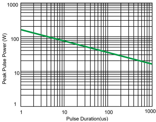
Fig 3. Non-Repetitive Peak Pulse Power vs. Pulse time
