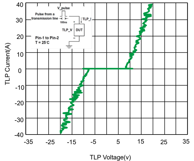
Fig 6. TLP Measurement
