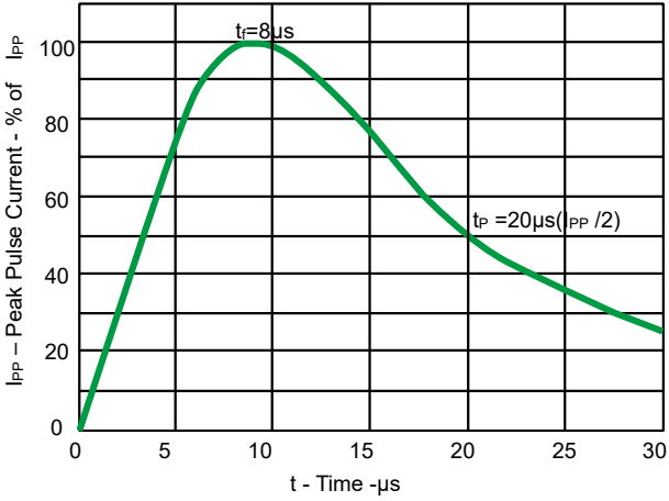
Fig 1. Pulse Waveform
