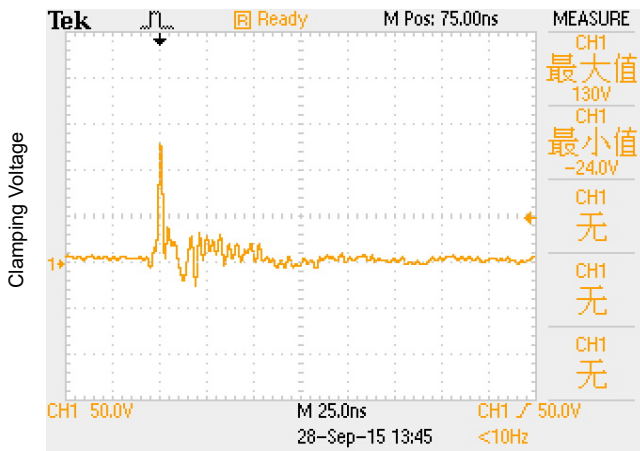
ESD clamping
