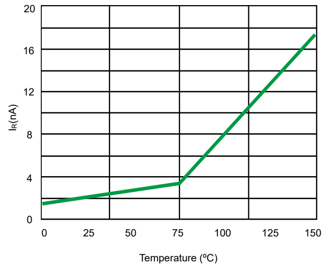
Fig 4. Typical Leakage Current vs. Temperature
