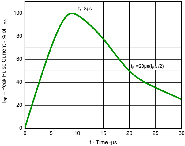
Fig 1. Pulse Waveform(8/20µs)
