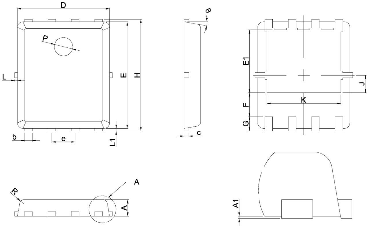
DETAIL "A"
