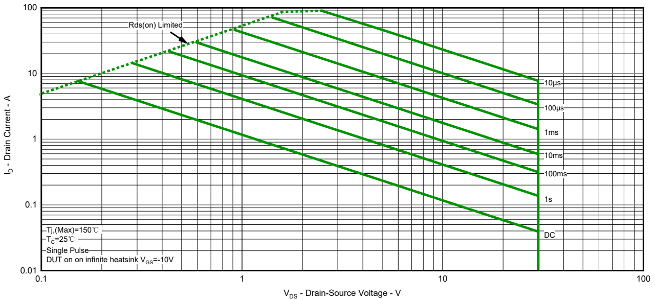
Fig.9 Safe Operation Area
