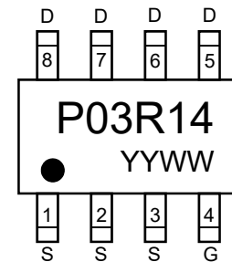
Marking (Top View)
