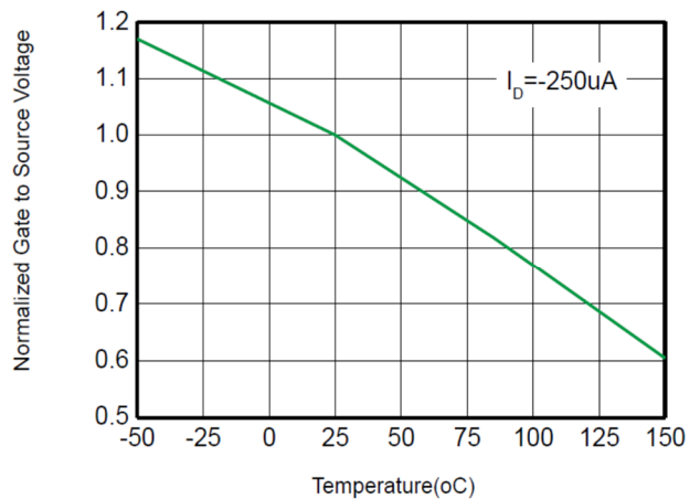
Fig 6. Threshold voltage vs. Temperature
