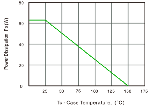
Fig.2 Power Dissipation
