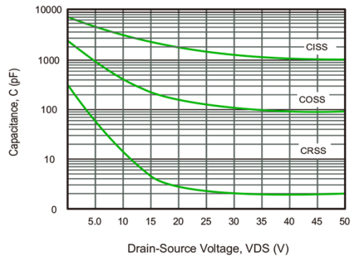
Fig.4 Capacitance Characteristics
