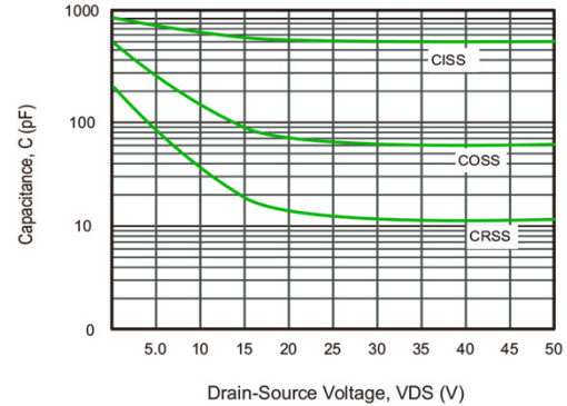
Fig.4 Capacitance Characteristics
